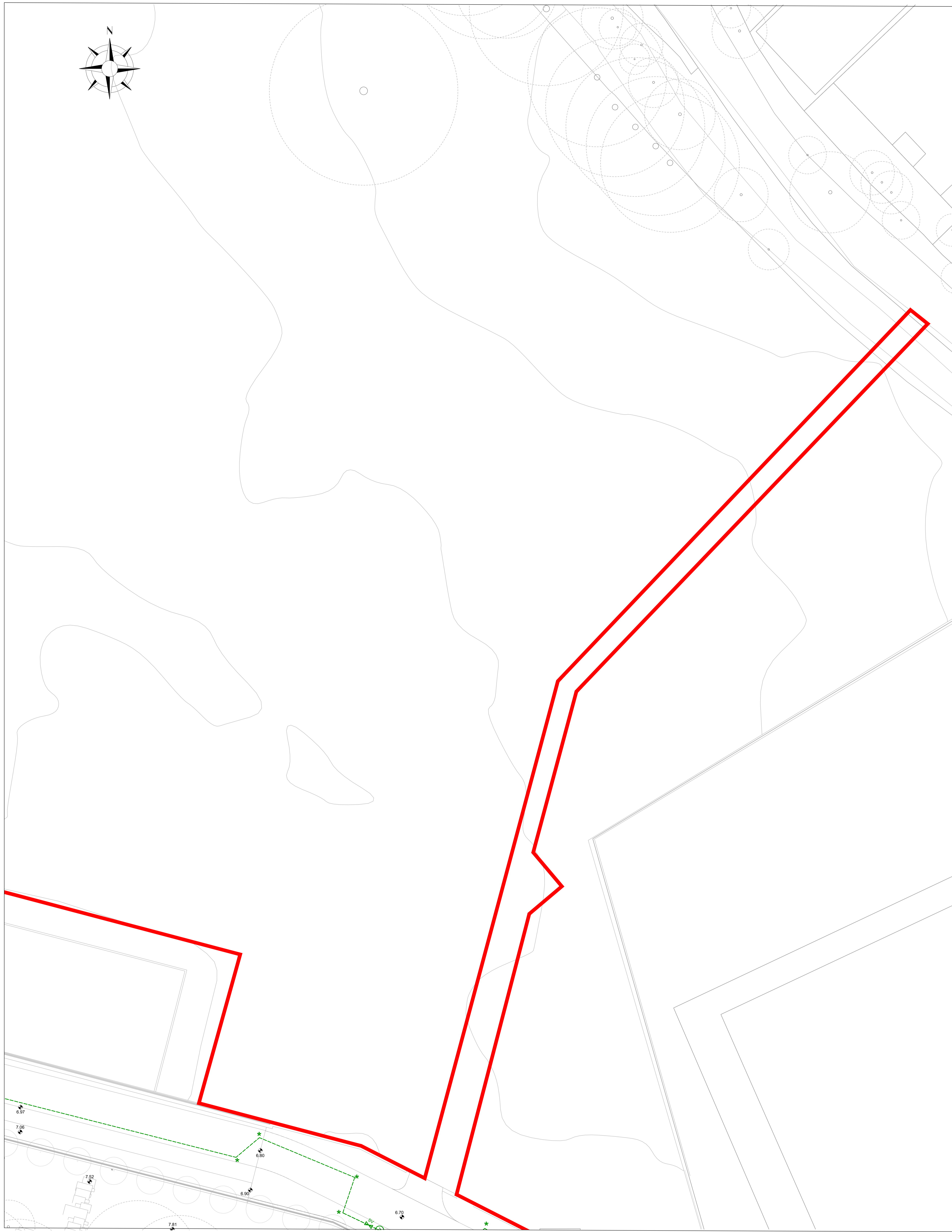
PROPOSED WATERMAIN SITE PLAN LAYOUT - SHEET 7 OF 8 SCALE @ A0: 1:200 SCALE @ A2: 1:400
